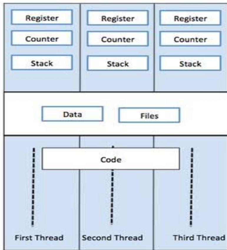
Single Process P with three threads
